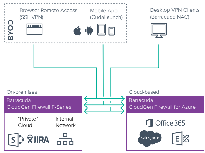
Figure 3 - Remote Access via VPN
