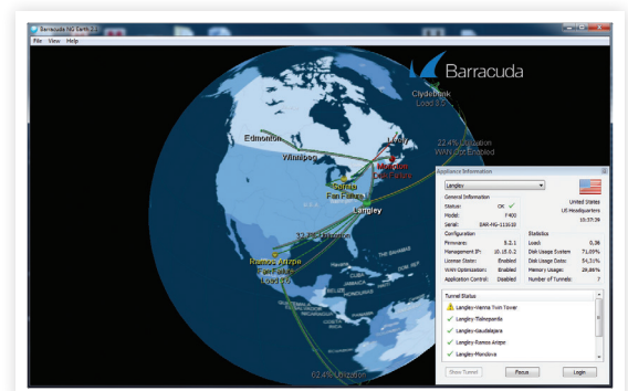
Barracuda Earth - the graphical real-time 3D network monitoring utility of the Barracuda Firewall Control Center, provides a status overview of all VPN site-to-site tunnels.
